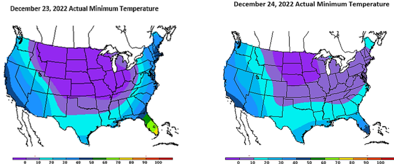
Figure 24: December 23 and 24, 2022 Actual Minimum Temperatures – Lower 48
