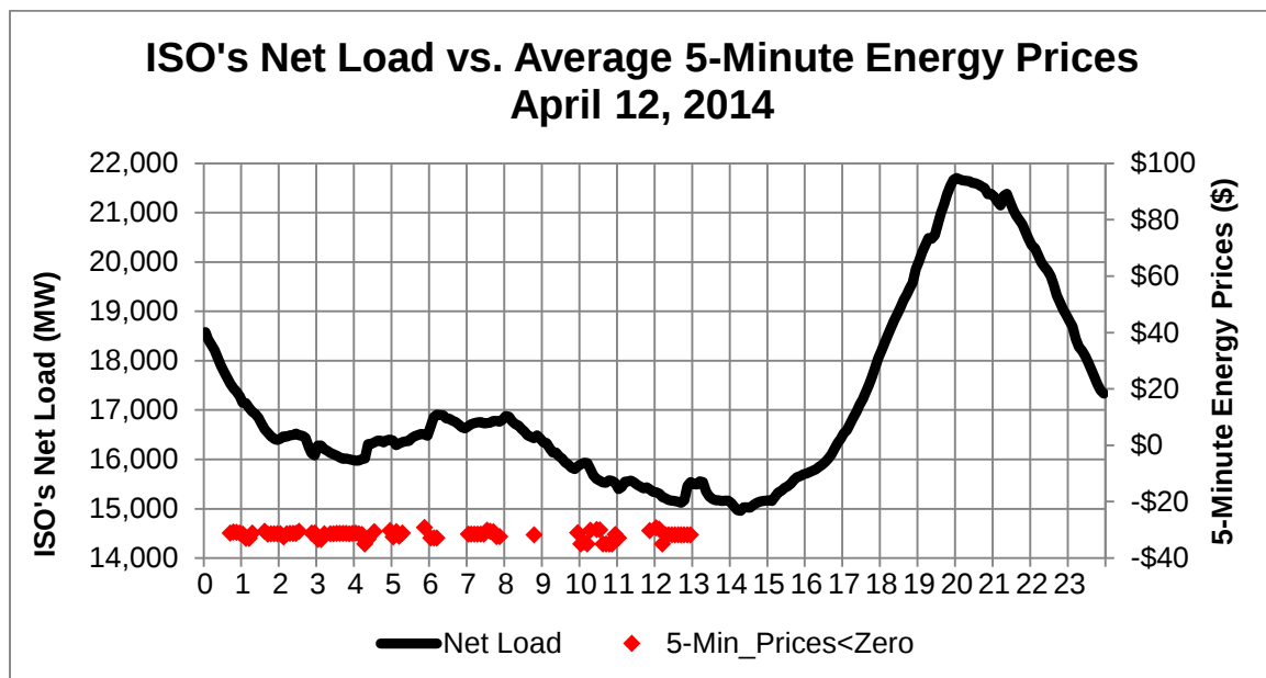
Figure 1 - Actual Net Load Curve for April 12, 2014
