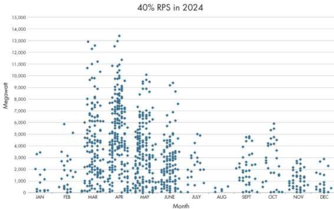
Figure 3: Estimated Renewable Curtailment Frequency and Magnitude in 2024 at 40% RPS
