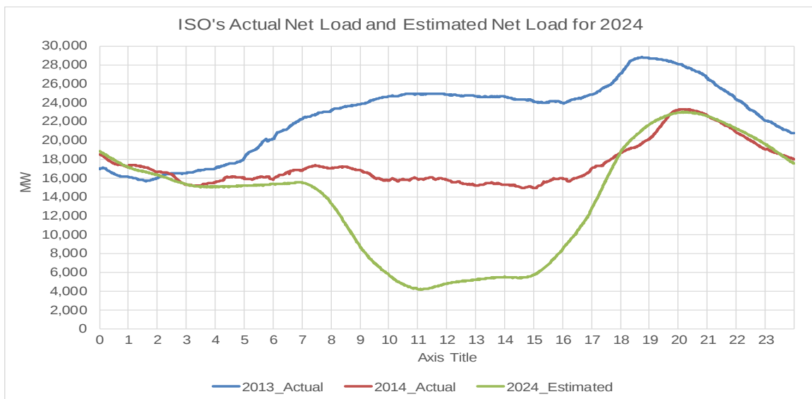
Figure 2: Net Load Curves (2013, 2014 and 2024 Estimated)
