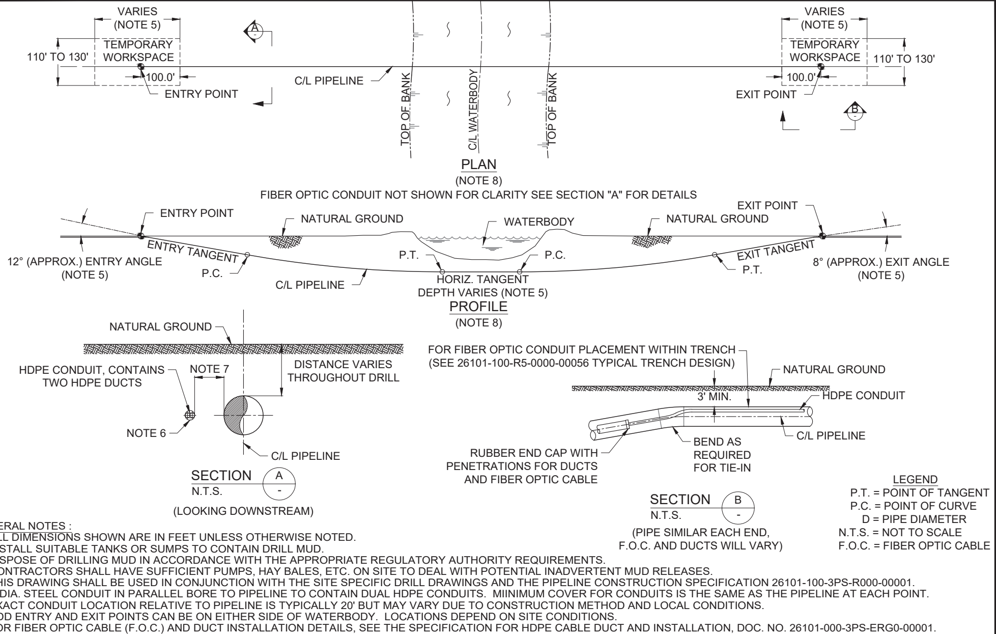
Figure 2.5-2 Typical HDD Crossing
