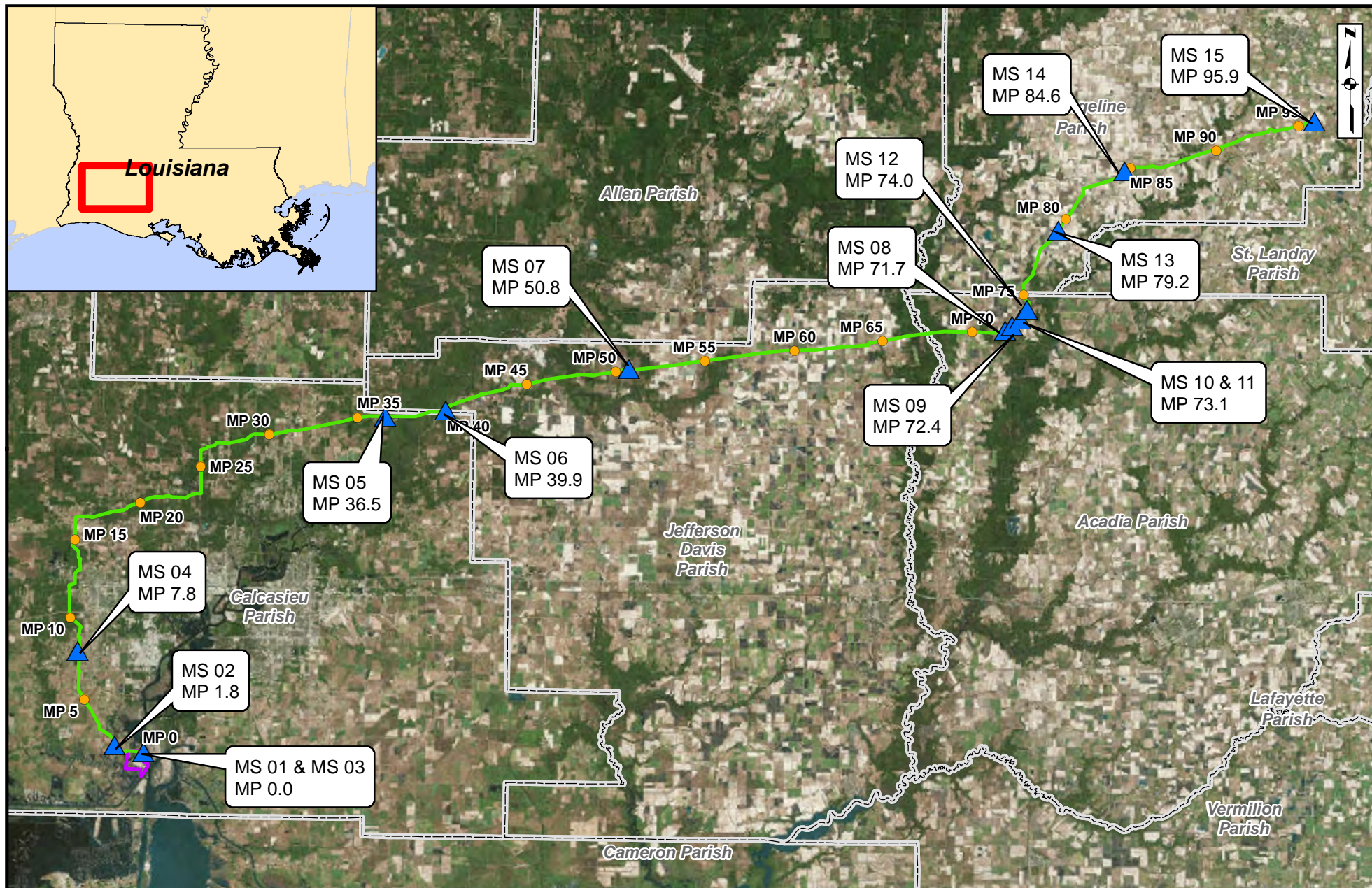
Figure 2.1-4: Meter Station Locations Map Driftwood LNG Project Driftwood LNG LLC and Driftwood Pipeline LLC Calcasieu, Jefferson Davis, Acadia, and Evangeline Parishes, Louisiana
