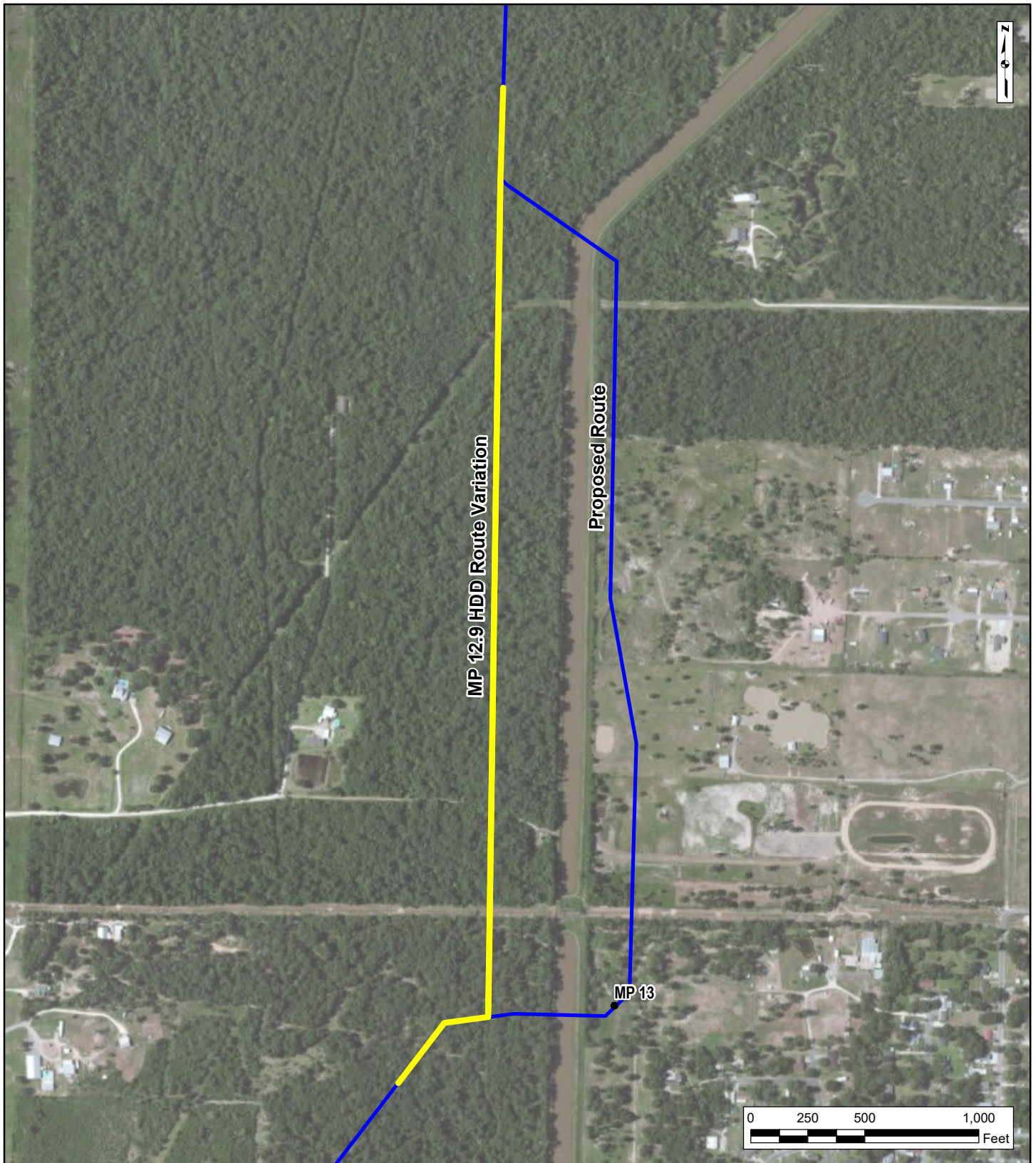
Figure 3.6-3: MP 12.9 HDD Variation Driftwood Project Calcasieu Parish, Louisiana
