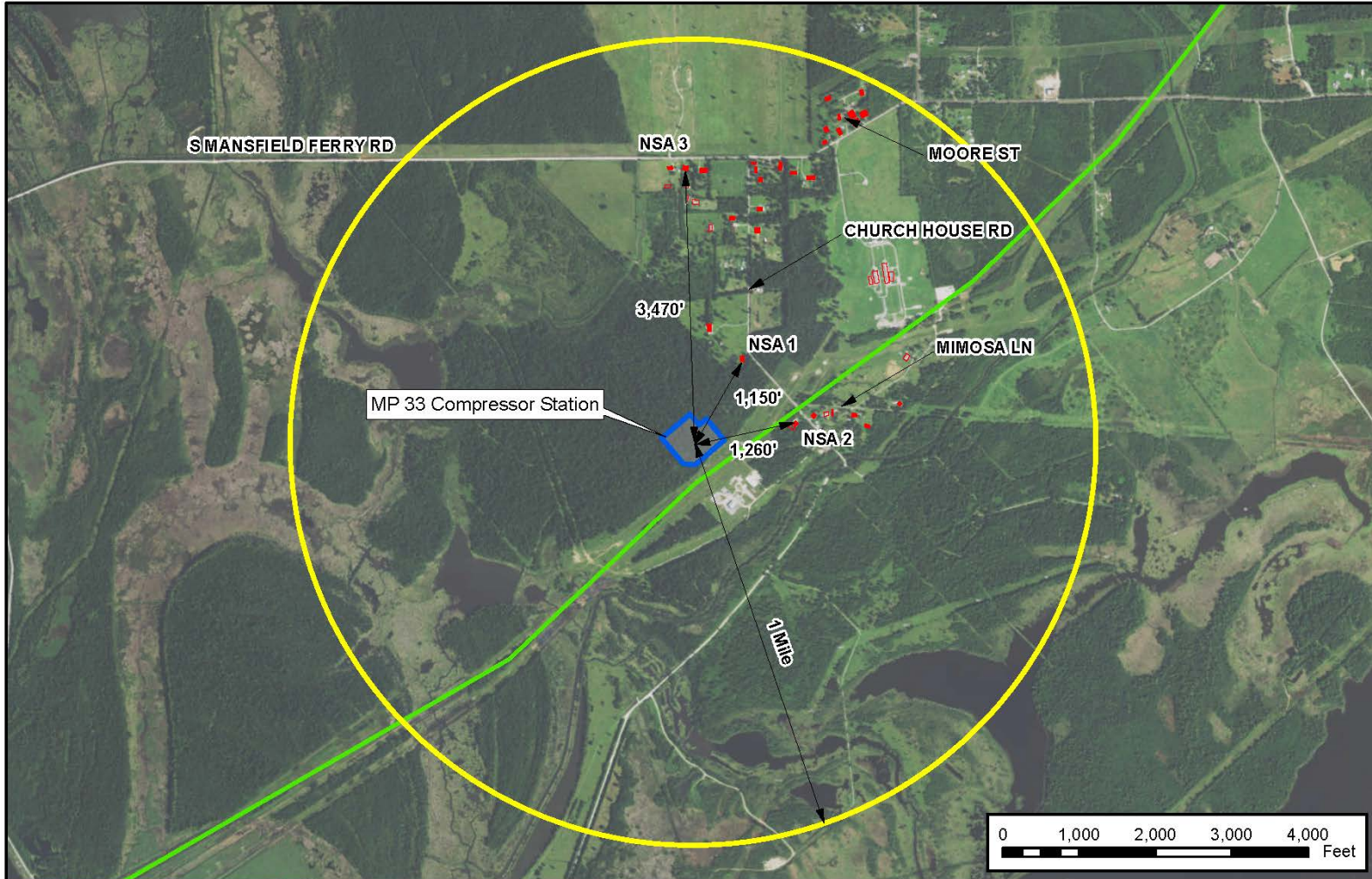
Figure 4.11.2-2 Golden Pass LNG Export Project NSAs for the MP 33 Compressor Station
