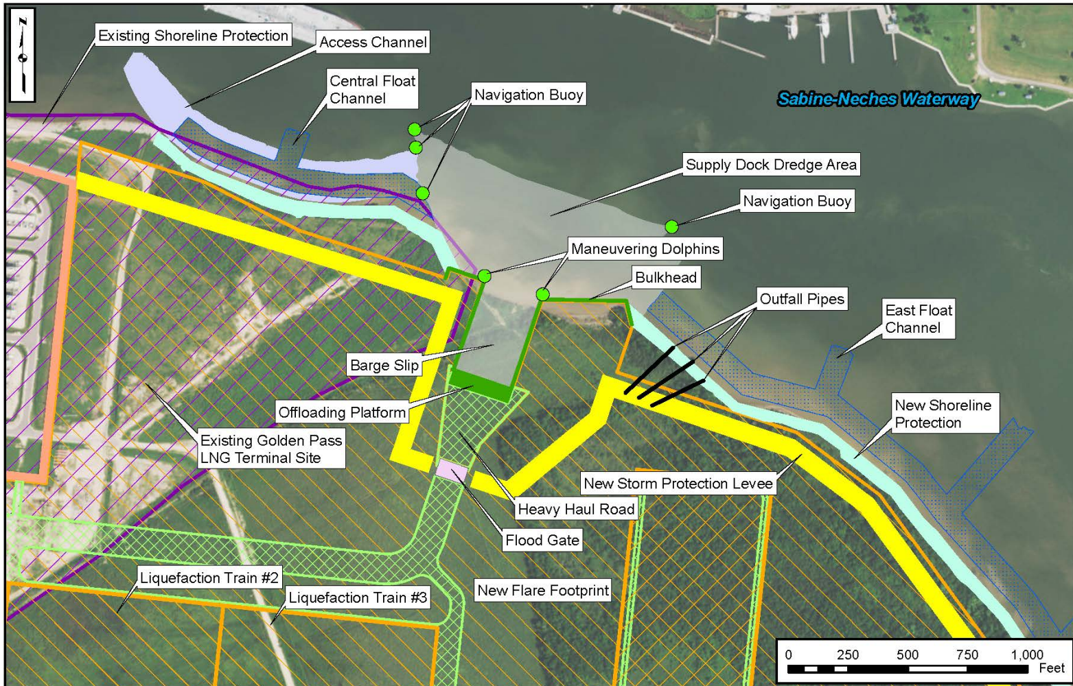
Figure 2.2-1 Golden Pass LNG Export Project Supply Dock
