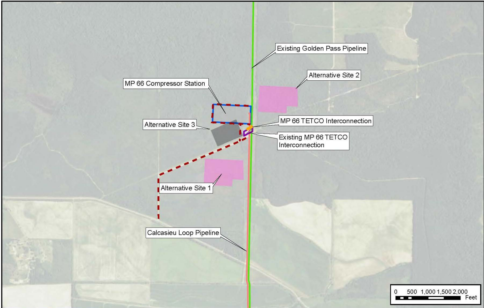
Figure 3.7-2 Golden Pass LNG Export Project Alternative Sites for the MP 66 Compressor Station
