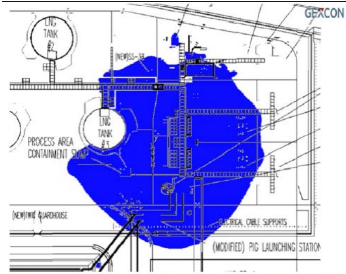
Figure 4.12.1-19 Maximum Extent of 1 psi from Mixed Refrigerant Scenario MR-136 from the Congested Area of Train 1 nearest to the LNG Storage Tanks (using an uncertainty factor of 2) (property line shown as a bold line in figure 4.12.1-17)
