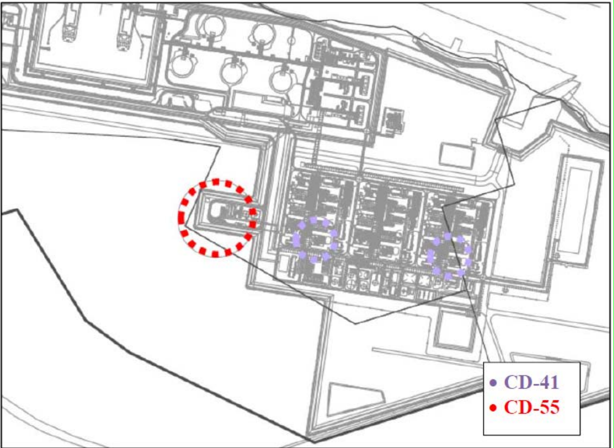
Figure 4.12.1-10 Maximum Flammable Vapor Dispersion from Hydrocarbon Condensate Design Spills ( property line shown in bold )
