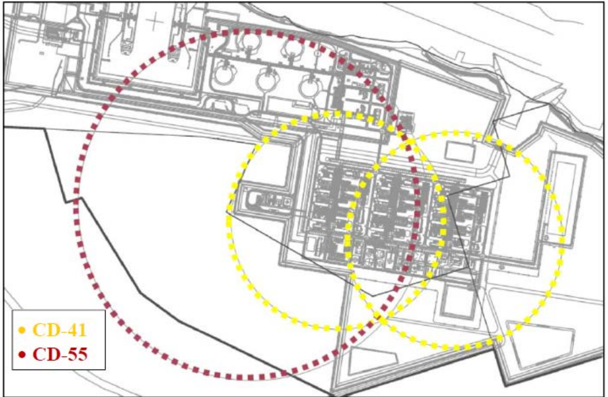
Figure 4.12.1-14 Maximum Distances to AEGL-1 for Benzene in the Condensate Design Spills ( property line shown in bold )
