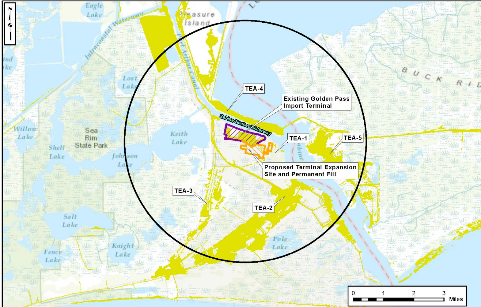
Figure 3.3-1 Golden Pass LNG Export Project Terminal Expansion Alternative Sites in Upland Areas
