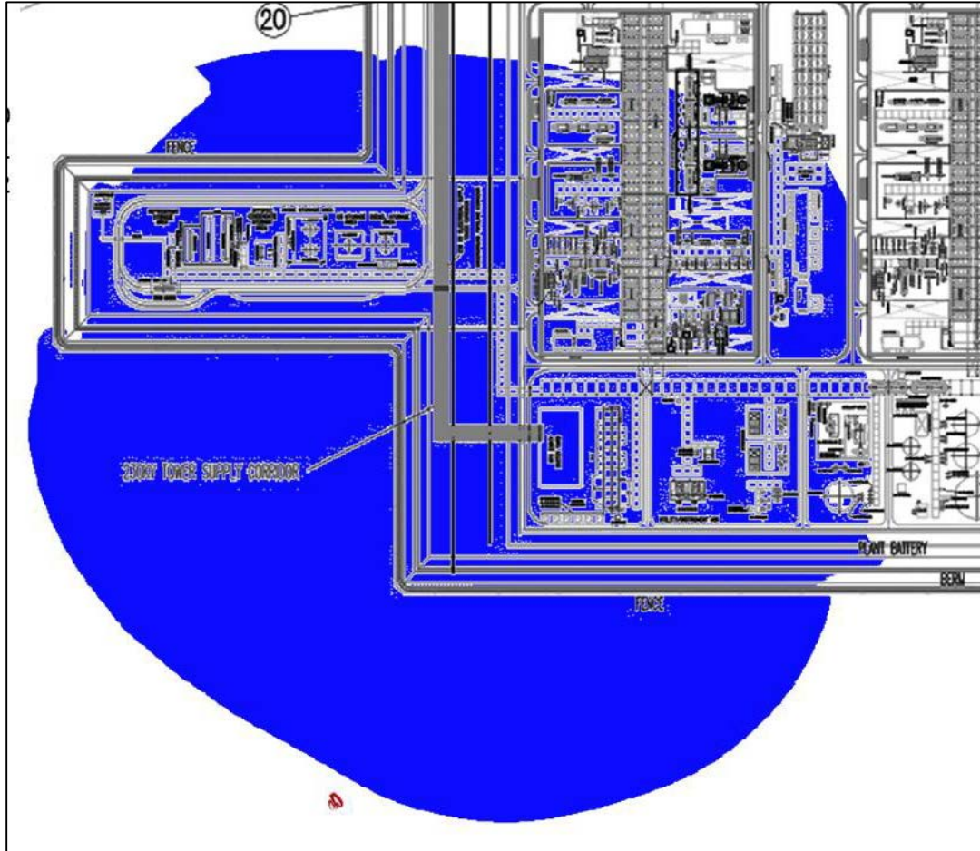
Figure 4.12.1-18 Maximum Extent of 1 psi from Condensate Overpressure Scenarios at the Southwest Corner of the Liquefaction Area ( using an uncertainty factor of 2 ) ( property line shown as a bold line in figure 4.12.1-17 )
