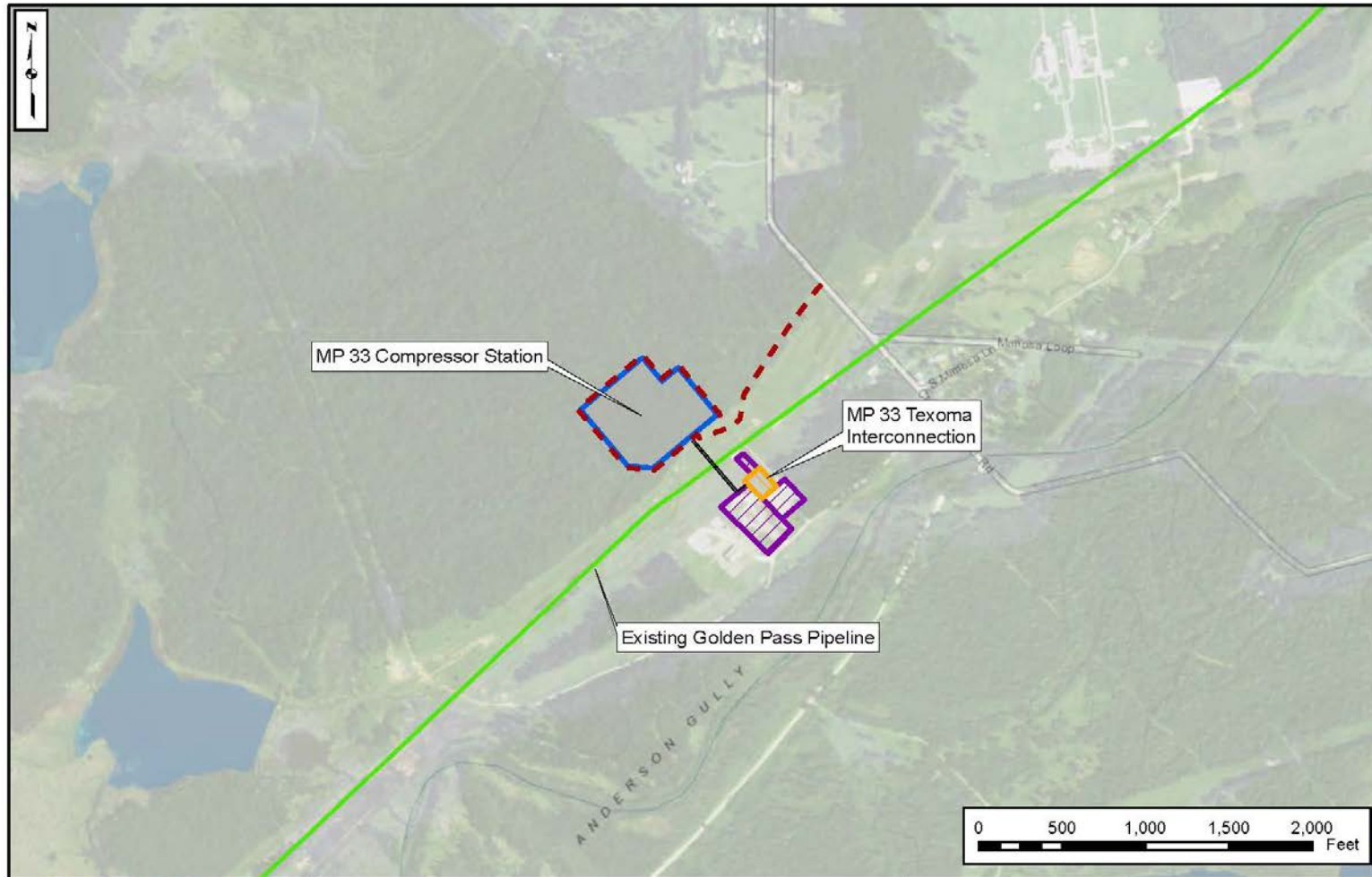
Figure 2.0-3 Golden Pass LNG Export Project Pipeline Expansion Route and MP 33 Facilities
