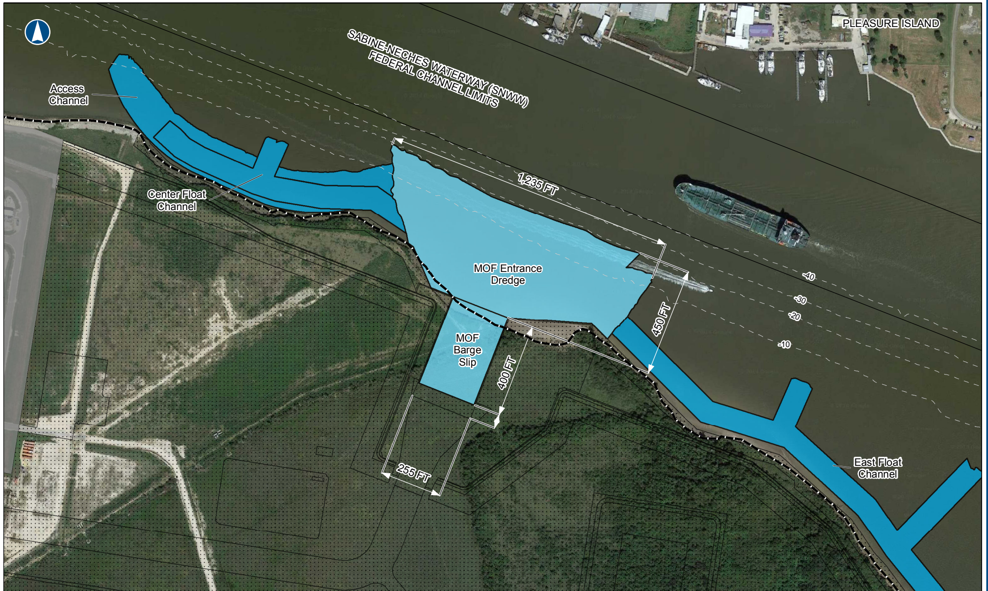
FIGURE 2-2 : MOF DREDGE AREAS
