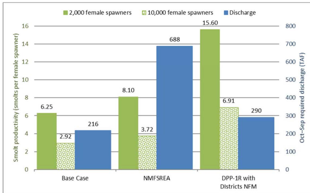
Figure 3.3.2-26. Average annual fall-run Chinook smolt production and required instream flows under base case, NMFS’s flow recommendation, and the Districts’ proposal (including the Districts’ non-flow measures) (Source: Districts, 2018a).
