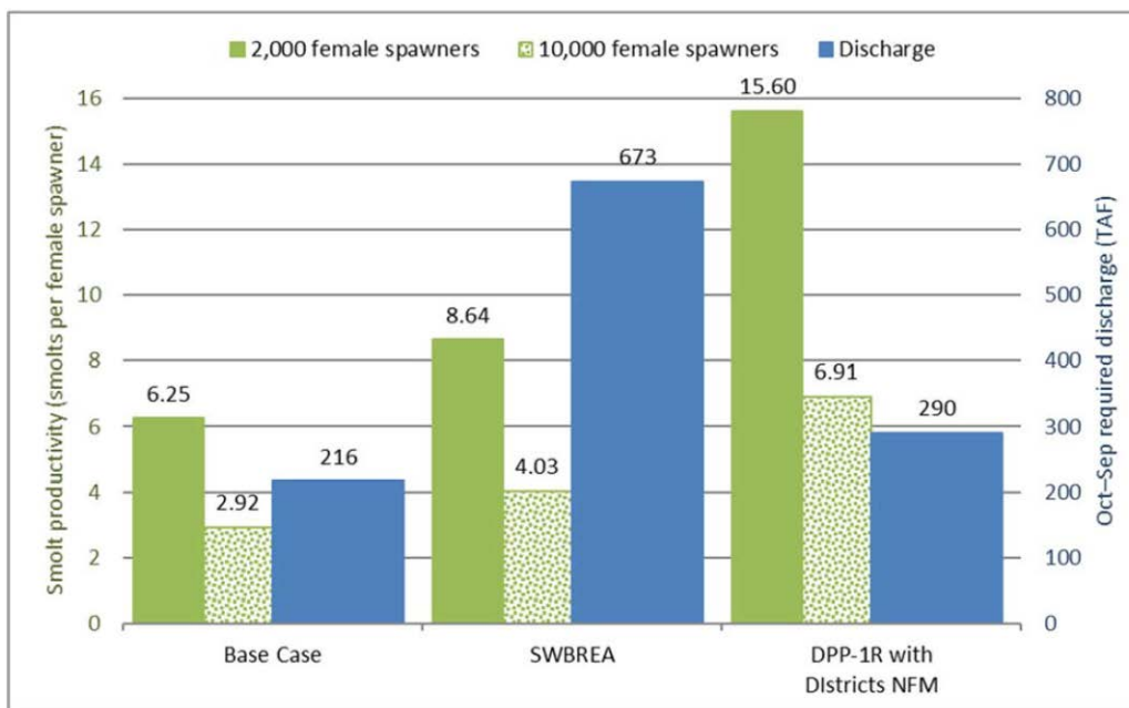
Figure 3.3.2-32. Average annual fall-run Chinook smolt production and required instream flows under the base case, the Water Board's flow recommendation, and the Districts' proposal (including the Districts' non-flow measures) (Source: Districts, 2018a).
