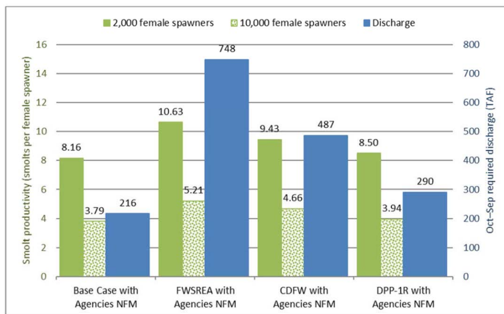
Figure 3.3.2-38. Estimated effects on Tuolumne River fall-run Chinook smolt production using base case instream flows, FWS's recommended instream flows, California DFW's instream flows, and the Districts' proposed instream flows when combined with agency/ Conservation Groups' non-flow measures of coarse sediment augmentation, floodplain lowering, and LWM augmentation (Source: Districts, 2018a).
