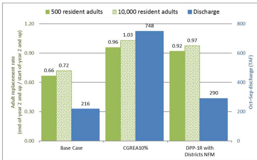
Figure 3.3.2-37. Average annual O. mykiss adult replacement rate for base case, the Conservation Groups' flow recommendation, and the Districts' proposal (including the Districts' non-flow measures) (Source: Districts, 2018a).
