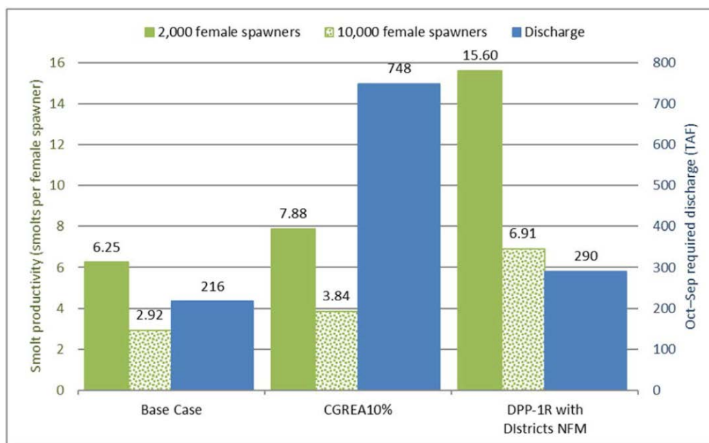
Figure 3.3.2-35. Average annual fall-run Chinook smolt production and required instream flows under the base case, the Conservation Groups' flow recommendation, and the Districts' proposal (including the Districts' non-flow measures) (Source: Districts, 2018a).
