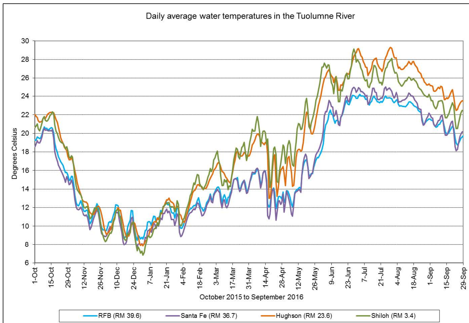
Figure 3.3.2-7. Tuolumne River daily mean temperature between RM 39.6 and RM 3.4, water year 2016 (Source: Districts, 2017c).
