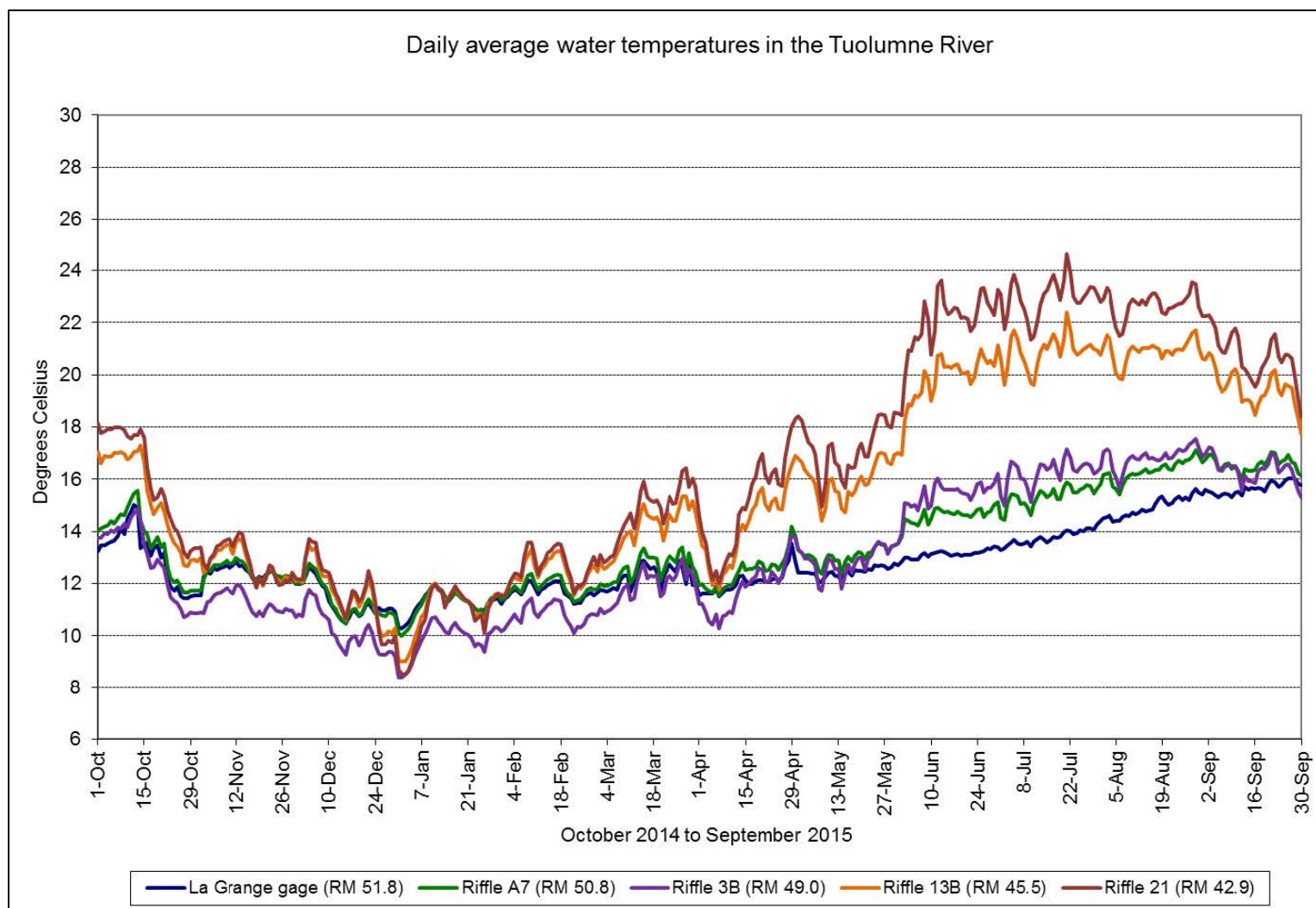
Figure 3.3.2-4. Tuolumne River daily mean temperature between RM 51.8 and RM 42.9, water year 2015 (Source: Districts, 2016).
