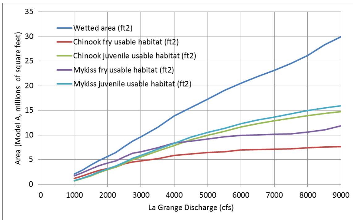
Figure 3.3.2-43. Model A results showing total wetted and usable habitat areas for juvenile salmonid life stages in the lower Tuolumne River (RM 51.7–RM 40) (Source: HDR and Stillwater Sciences, 2017).
