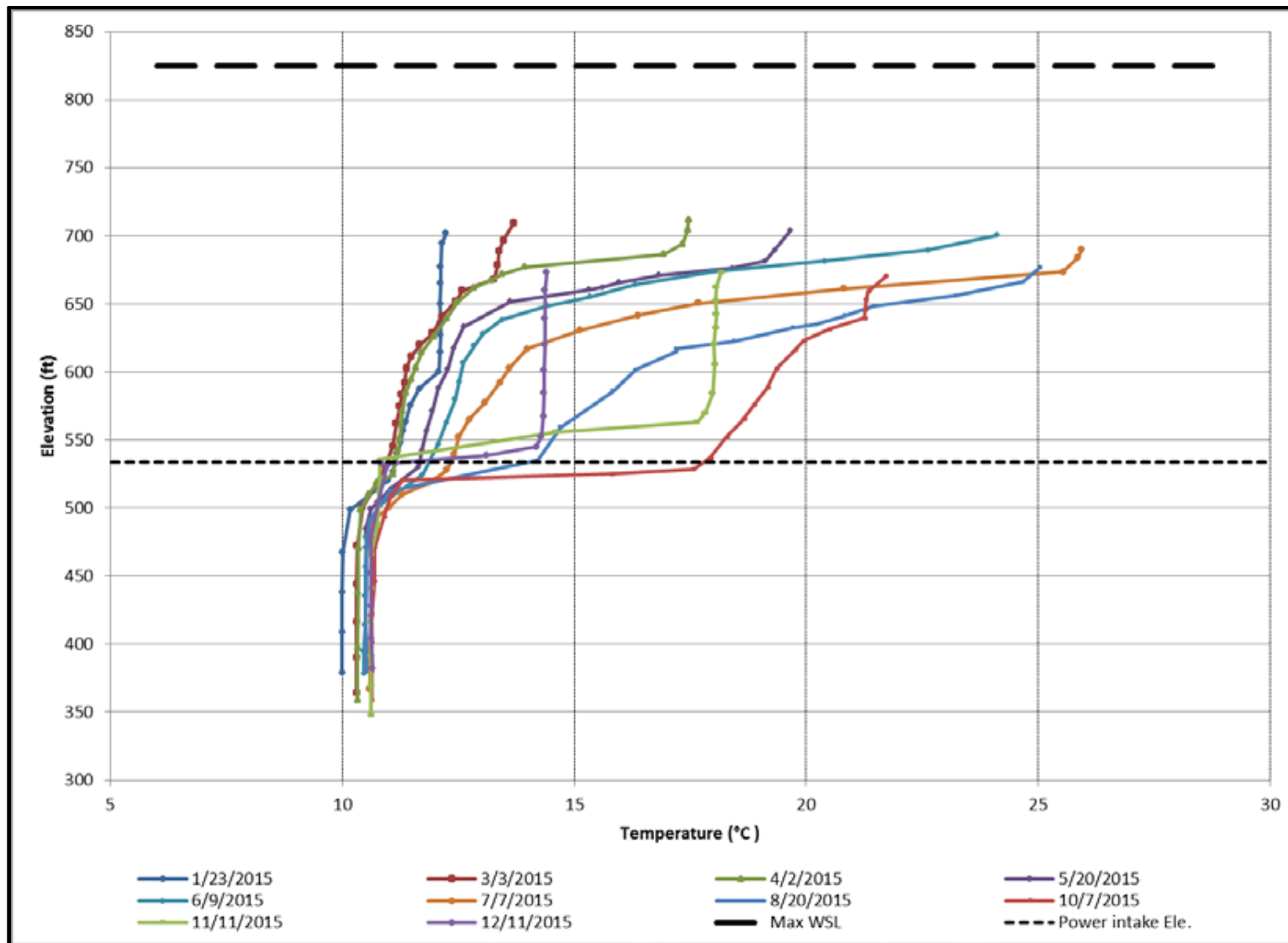
Figure 3.3.2-2. Water temperature profiles recoded in Don Pedro Forebay in 2015 (Source: Districts, 2017a).
