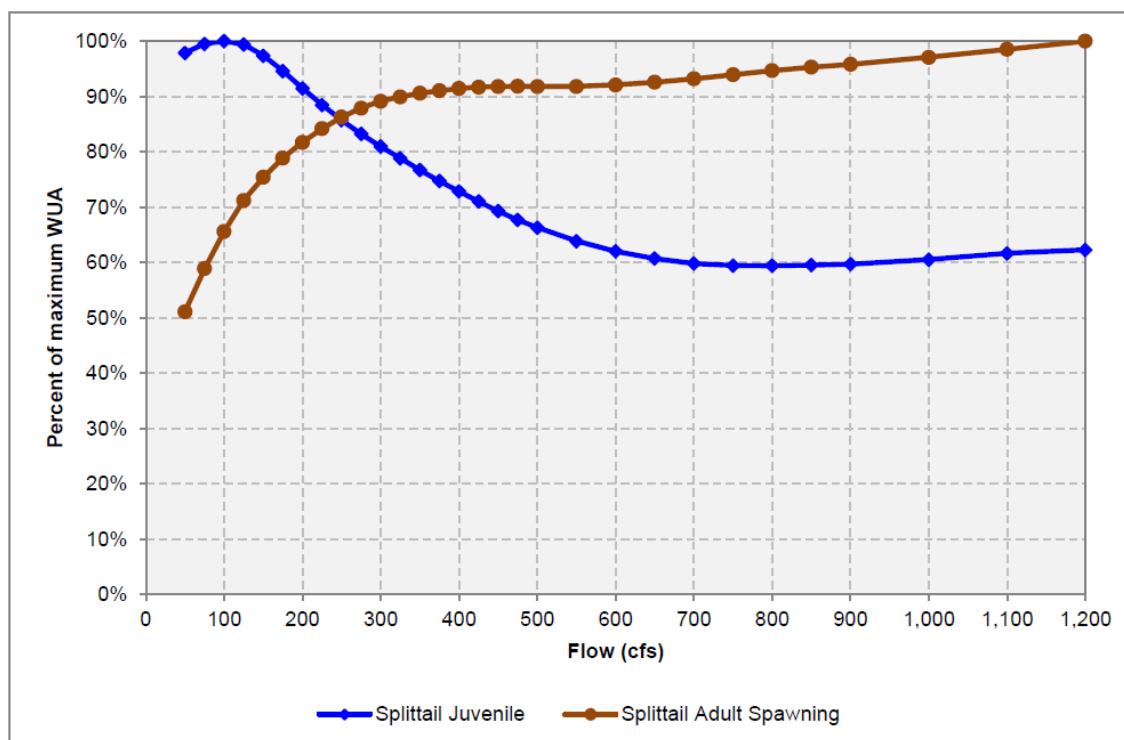
Figure 3.3.2-22. Sacramento splittail WUA results (percent of maximum) for the lower Tuolumne River (Source: Stillwater Sciences, 2014).
