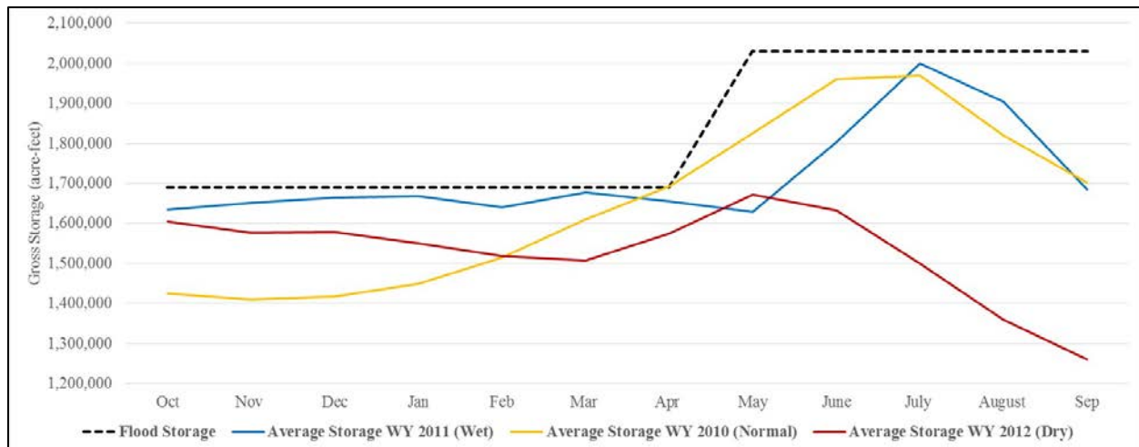
Figure 3.3.2-1. Don Pedro Reservoir storage curves for water years 2010–2012 (Source: USGS, 2018b).
